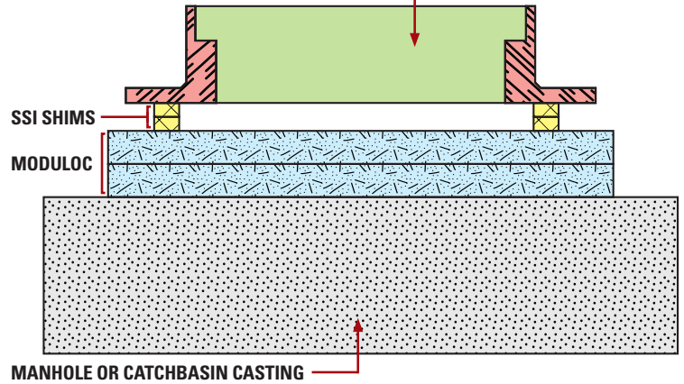
MANHOLE OR CATCHBASIN FRAME & GRATE
