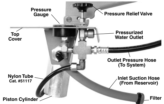
Figure 2 – Pump Components
