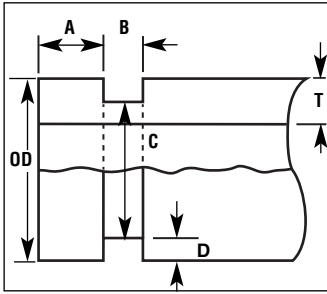
Figure 4 – Cut Groove Dimensions
