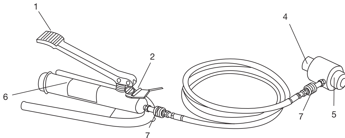
746A Hydraulic Ram with 1725 Foot Pump
