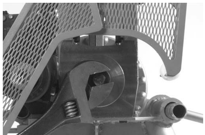
Figure 21 – Loosening The 5/8" Draw Bolt
