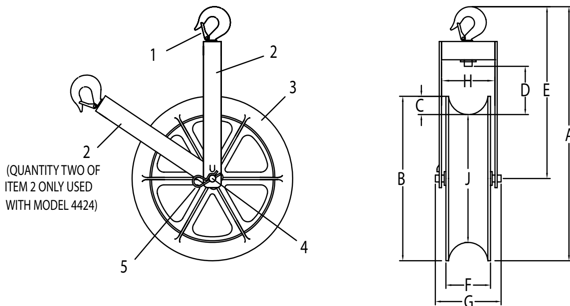
DIMENSIONAL CHART
