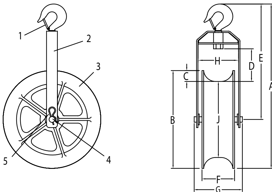
DIMENSIONAL CHART
