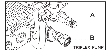
TRIPLEX PUMP
