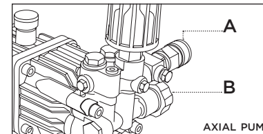
AXIAL PUMP
