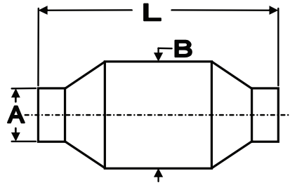
WELDED DESIGN
