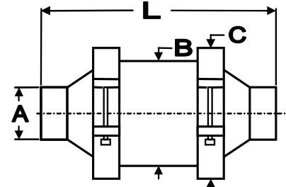
CLAMPED DESIGN
